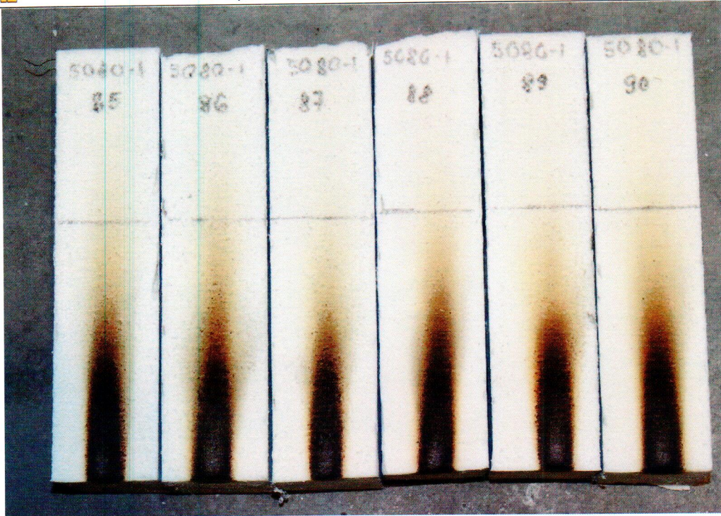
Fig.4. Specimens with 60 mm thickness after tests.
